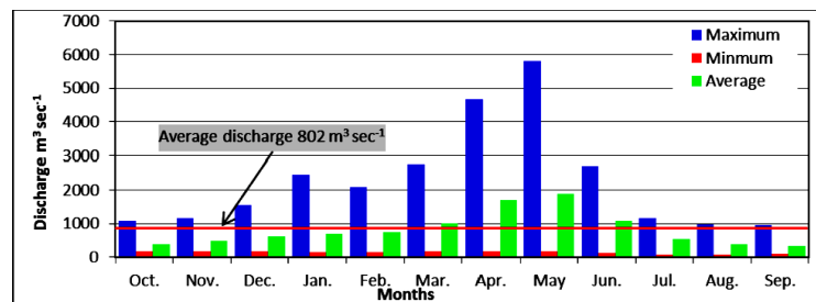
Figure 3. Monthly (mean, maximum and minimum) discharge of Euphrates River at Hit site (1932-1997).
