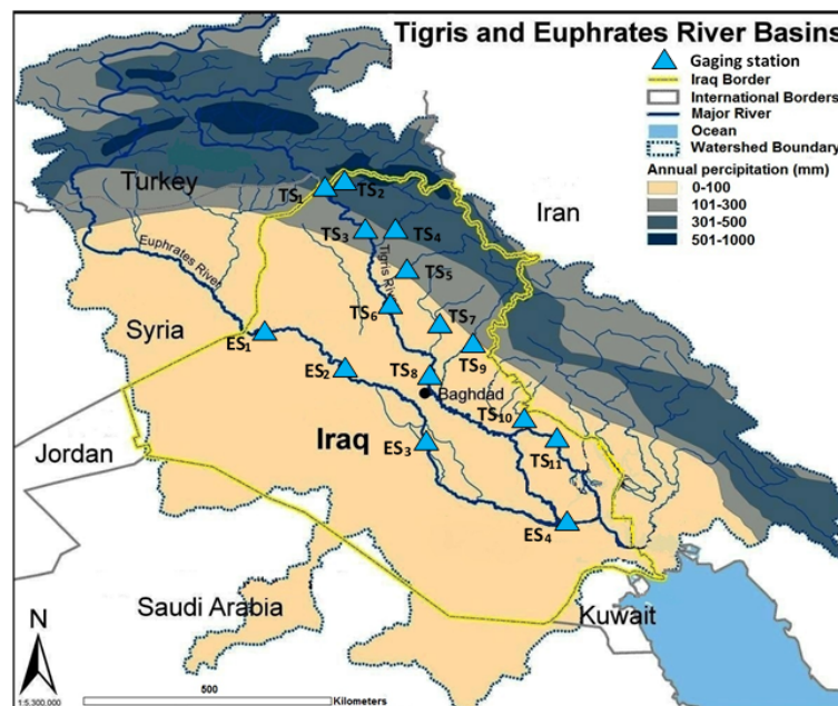
Figure 1. General layout of the Tigris-Euphrates Rivers and locations of stream flow gaging stations.
