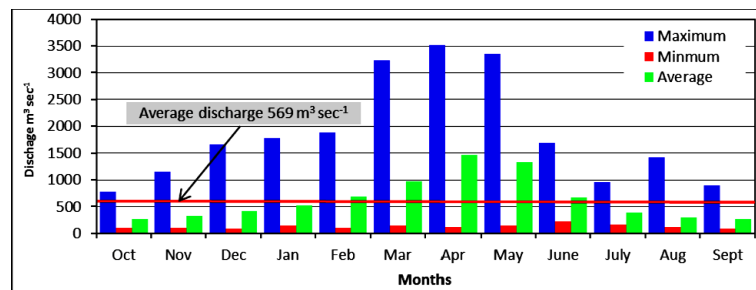
Figure 2. Monthly (mean, minimum and maximum) discharge of Tigris River at Mosul dam site (1931-2011).
