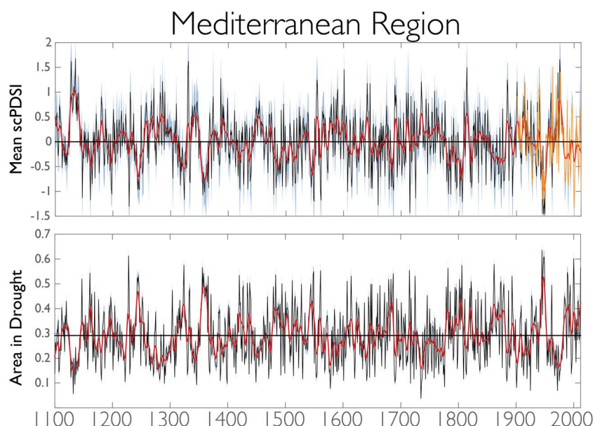
Figure 4. (top) Area average scPDSI for the entire Mediterranean domain in the OWDA (30°N–47°N, 10°W–45°E) and (bottom) percent land area in drought (scPDSI \leq -1 ) from 1100 to 2012 C.E. Red curves are smoothed versions of the time series using a 10 year loess smooth. In Figure 4 (top), regional average scPDSI calculated from the instrumental target data set for the OWDA reconstruction is overlain in orange. The horizontal line in Figure 4 (bottom) is the long-term average fractional area in drought from 1100 to 2012 C.E. (29%). Grey-blue shading indicates the 95th confidence intervals, estimated using a BCa bootstrap.
