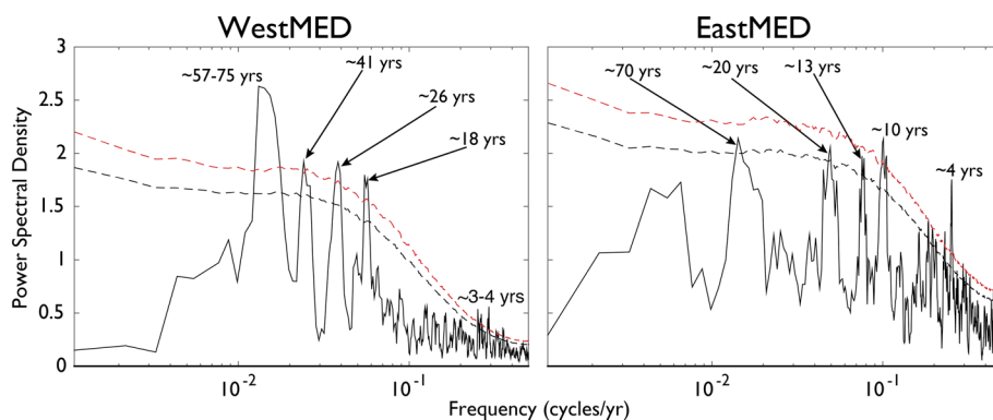
Figure 8. Power spectral density (multitaper method, three tapers) for the WestMED and EastMED regional average scPDSI series. Red and black dashed lines are the 95th and 90th percentile confidence limits, respectively, estimated from 10,000 AR(1) series generated from the original time series.
