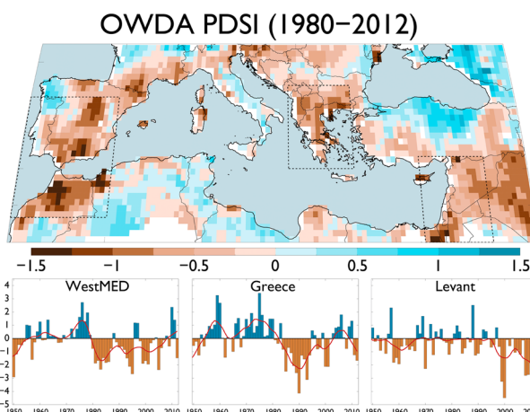
Figure 11. (top) Multiyear average scPDSI for 1980–2012 with regions of recent and persistent drought outlined in dashed black lines: WestMED (32°N–42°N, 10°W–0°), Greece (36°N–43°N, 19°E–26°), and the Levant (30°N–37°N, 33°E–40°E). (bottom) Also shown are the regional average scPDSI time series from these regions for 1950–2012 (red line is a 10 year loess smoother).
