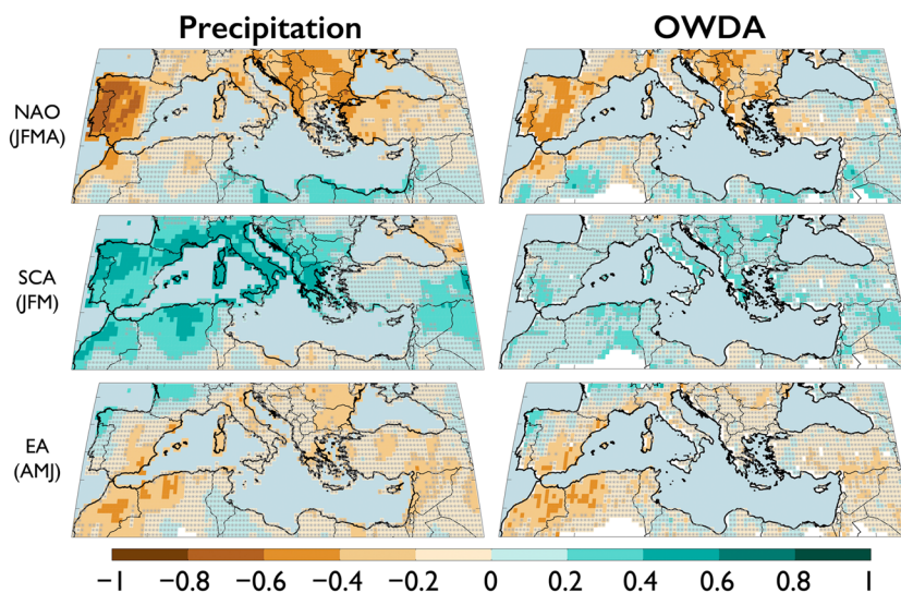
Figure 3. Spearman's rank correlation coefficients between the teleconnection indices (NAO, SCA, and EA) and (left column) simultaneous season CRU 3.21 precipitation totals and (right column) OWDA summer season scPDSI. Correlations are calculated over the period 1950–2012 C.E. Regions of insignificant correlation ( p > 0.05 ) are masked by grey asterisks.
