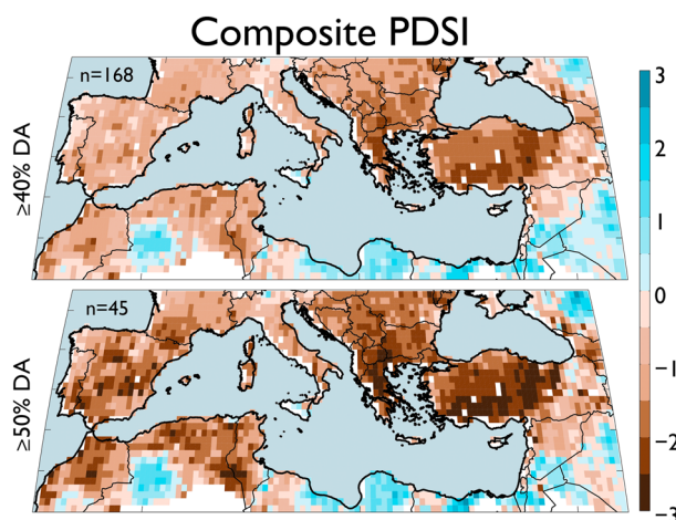
Figure 6. Composite average scPDSI for years in the OWDA with drought area (DA; scPDSI \leq -1 ) exceeding 40% ( n=168 years) and 50% ( n=45 years) of the total land area in the Mediterranean domain.
